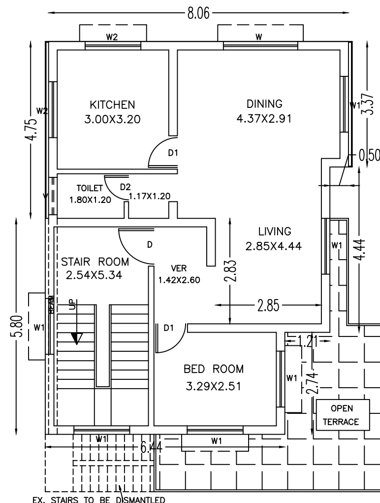
PROPOSED ADDITIONS TO THE EXISTING FIRST FLOOR PLAN
